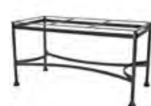
9-DT07 Dining Table Base Fits 42"x72", 42"x84" and 44"x84" Tops 28"H x 53.5"W x 26.5"D
